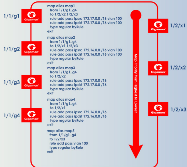
Figure 19-12: Sending Subnets and VLANs to Different Ports
