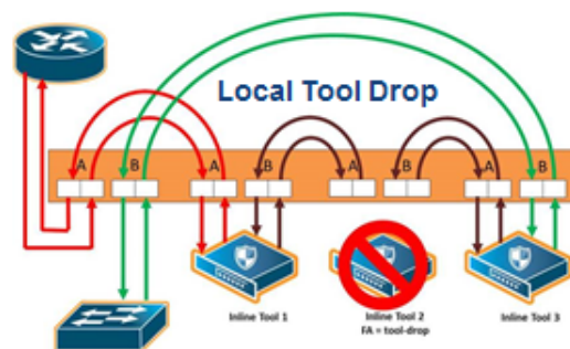
Figure 20-31: Inline Tool Series Local Tool Drop Failover Action
