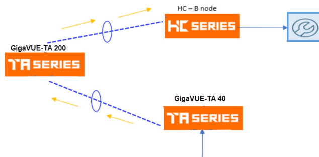
Figure 25-3: Multihop Topology
