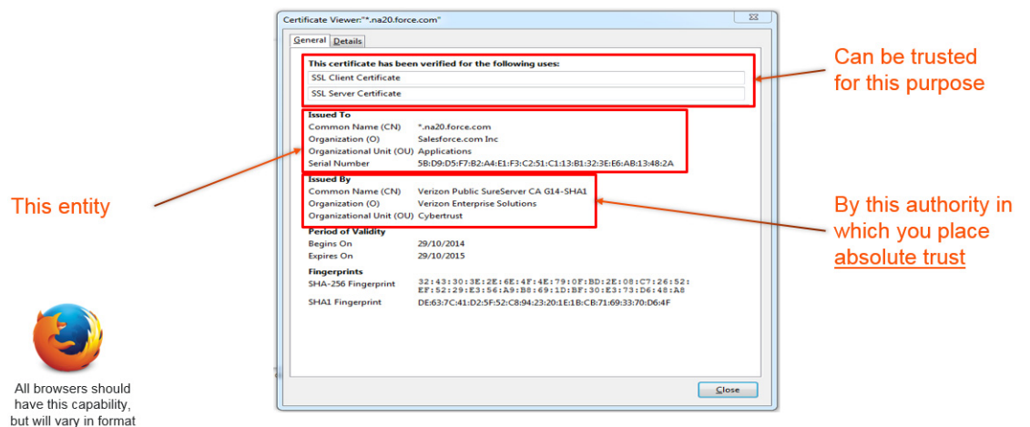
Figure 21-8: Sample Certificate
