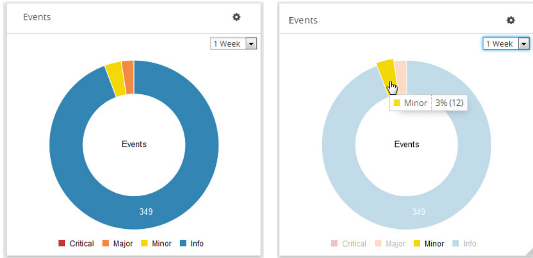
Figure 4-40: Events Widget
