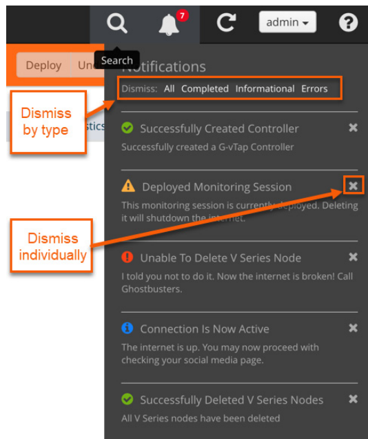
Figure 3-5: Long-term messages
