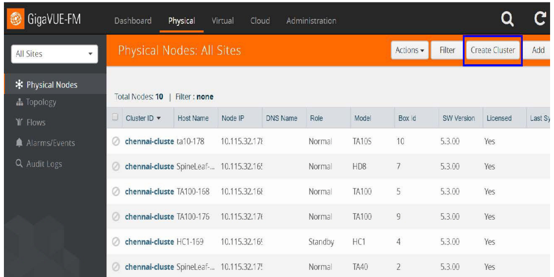
Figure 9-11: Create Cluster
