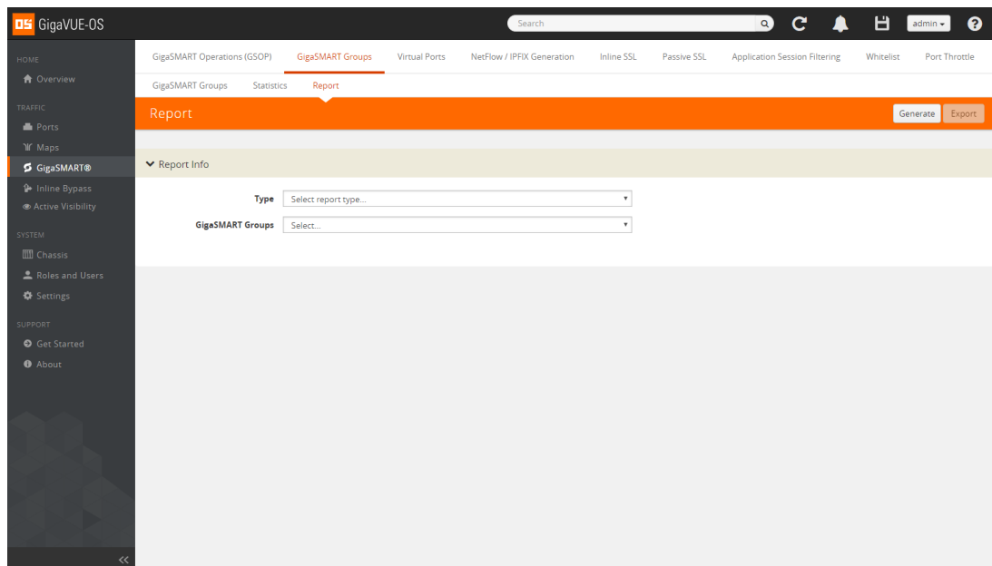
Figure 26-120: Report Page
