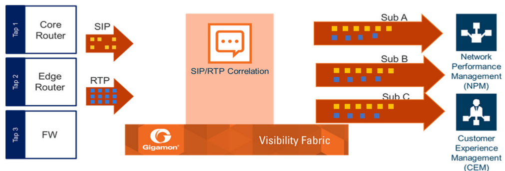
Figure 26-65: SIP/RTP Correlation
