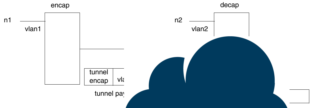
Figure 17-19: IP Interfaces
