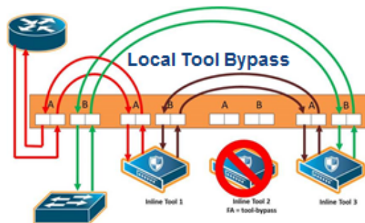
Figure 20-30: Inline Tool Series Local Tool Bypass Failover Action
