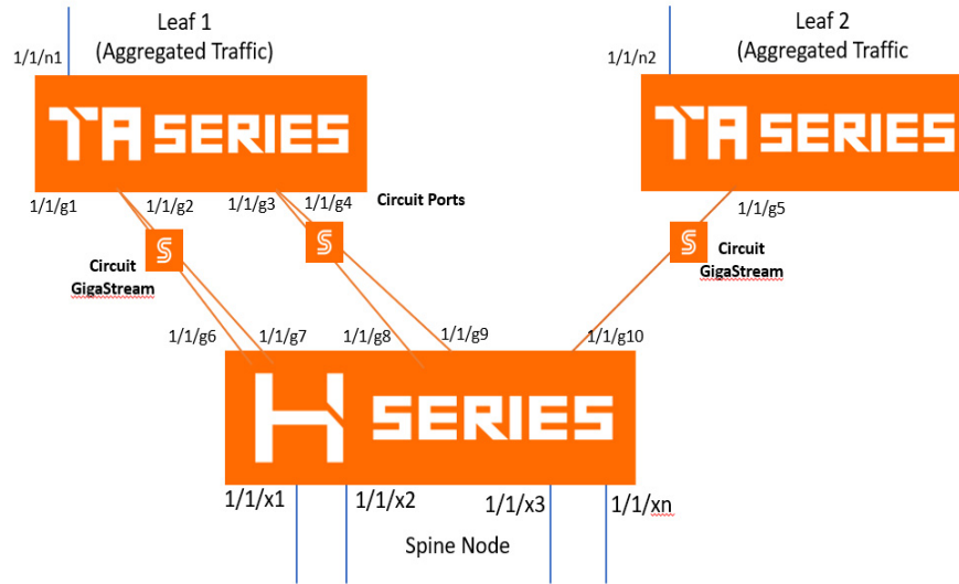
Figure 25-4: Circuit GigaStreams in Fabric Maps
