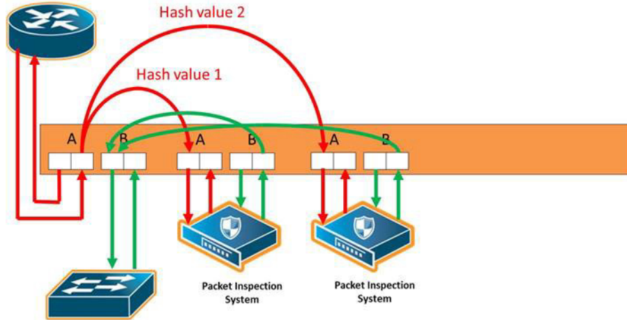
Figure 20-21: Inline Tool Group With No Spare, Non-Redundant
