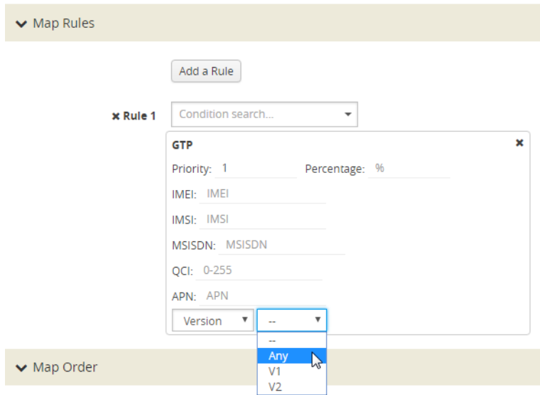
Figure 26-42: GTP Version
