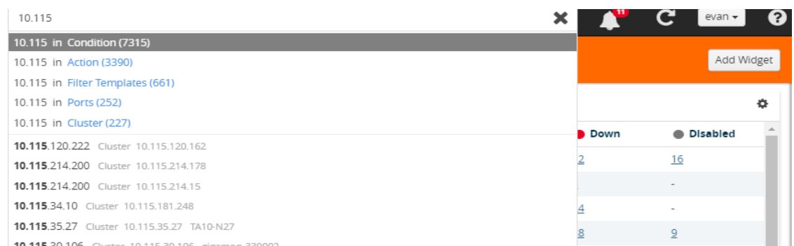
Figure 3-9: GigaVUE-FM Search
