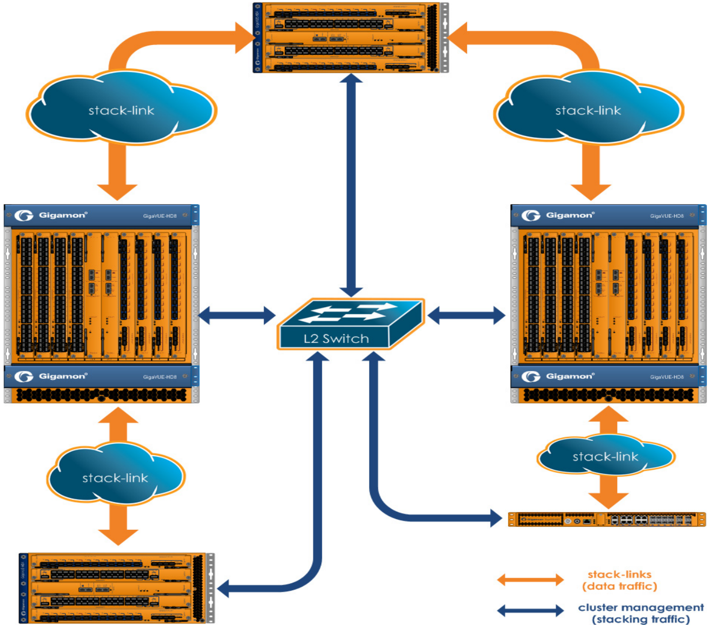
Figure 8-3: Sample Cluster
