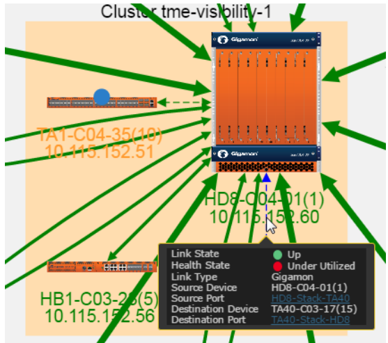
Figure 14-32: Link Information
