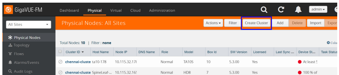
Figure 8-6: Create Cluster
