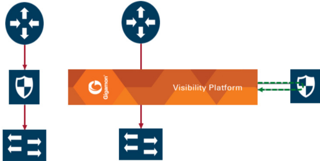
Figure 21-11: Simple Inline Tool Arrangement
