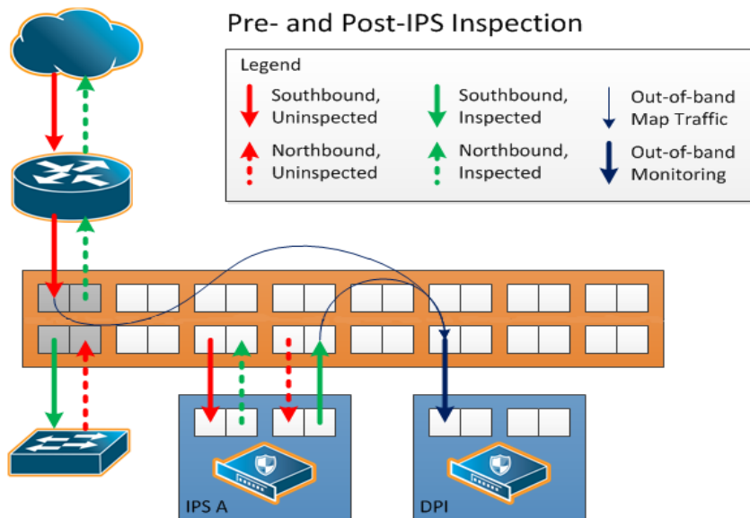
Figure 20-9: Out-of-Band Arrangement
