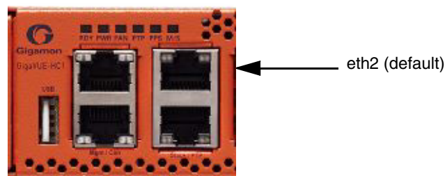
Figure 21-16: Stack Port Location on GigaVUE-HC1 Front
