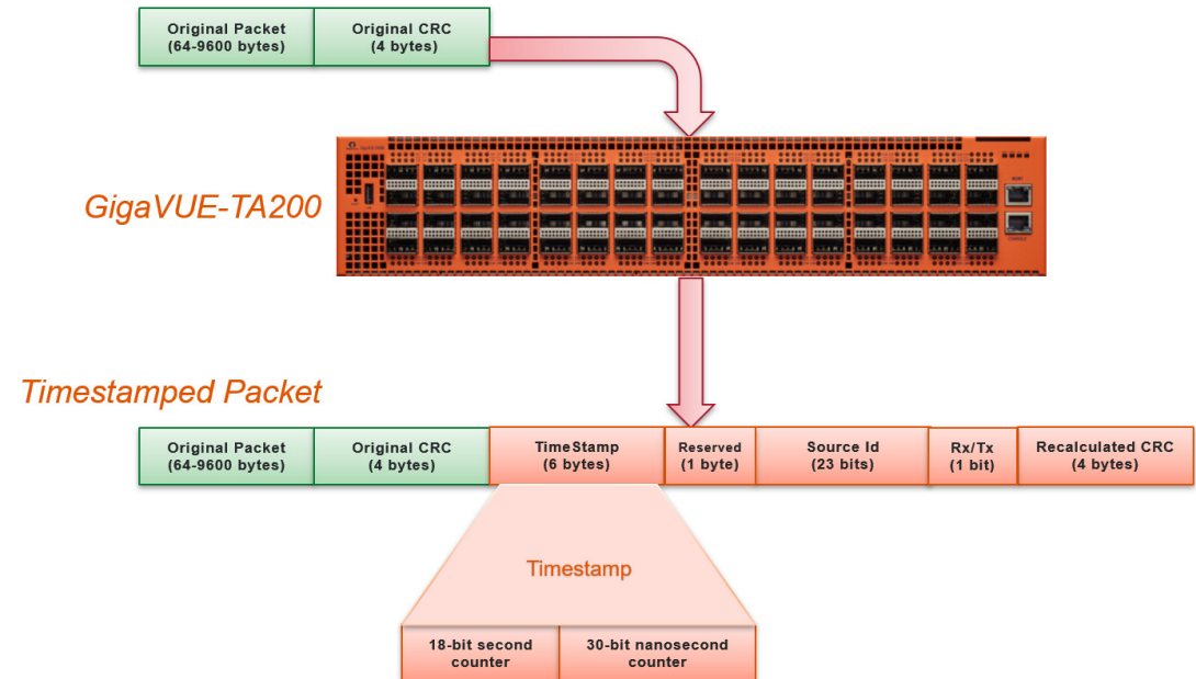
Figure 24-2: Timestamp Format
