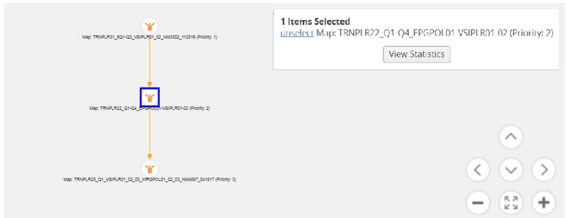
Figure 15-9: Maps Selected
