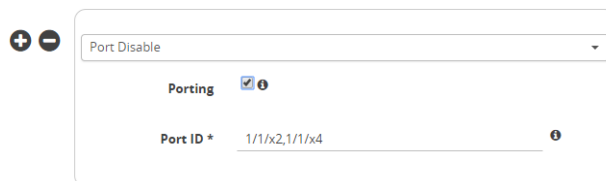
Figure 19-52: Port Actions
