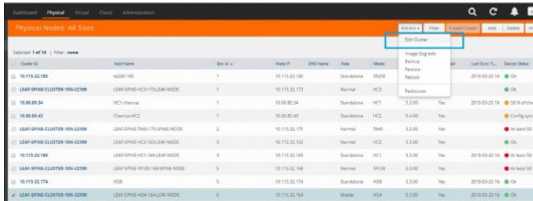
Figure 9-23: Edit cluster
