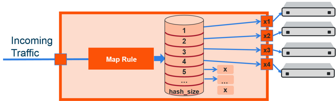
Figure 17-26: Controlled GigaStream Overview
