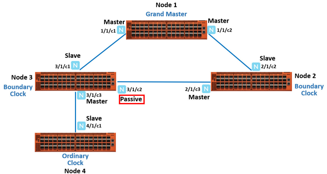
Figure 24-3: PTP Deployment
