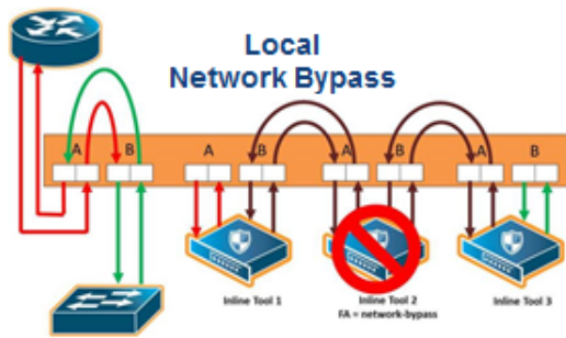
Figure 20-32: Inline Tool Series Local Network Bypass Failover Action
