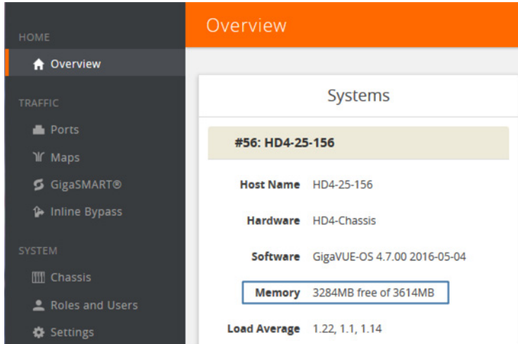
Figure 26-62: System Memory
