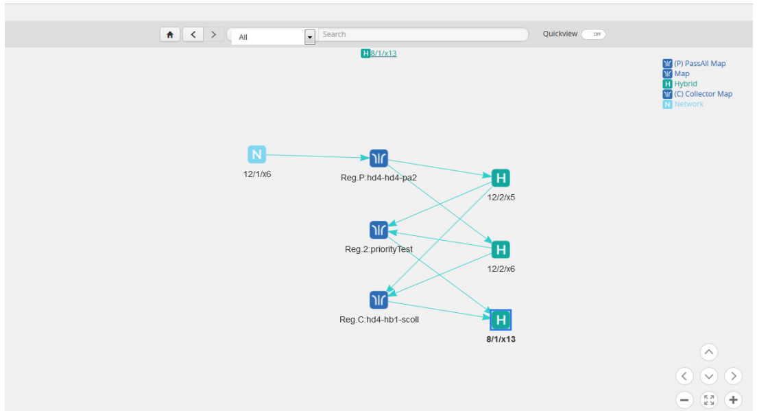
Figure 14-36: Map Selected
