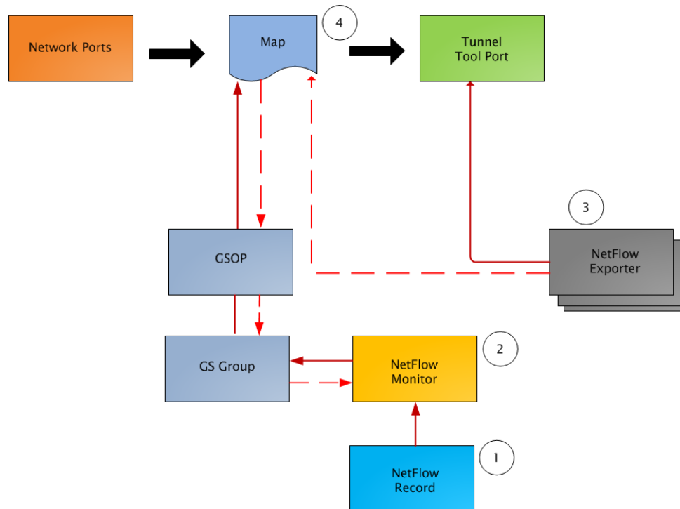
Figure 26-95: NetFlow Generation Components
