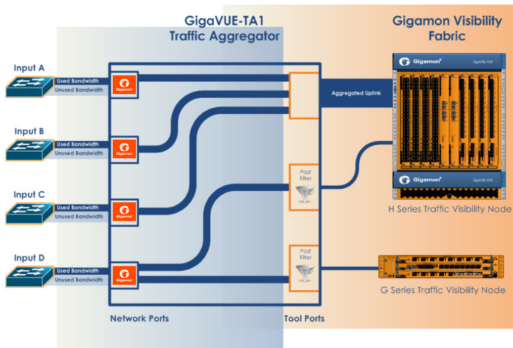
Figure 17-3: GigaVUE-TA1 Packet Distribution
