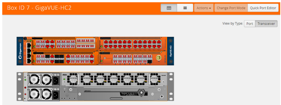
Figure 20-48: Chassis view of GigaVUE-HC2 with TAP-HC0-G100C0 Module
