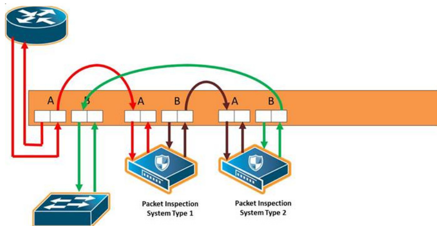
Figure 20-6: Inline Tool Series
