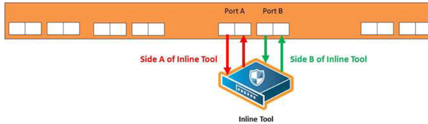
Figure 20-17: Inline Tool and Inline Tool Ports
