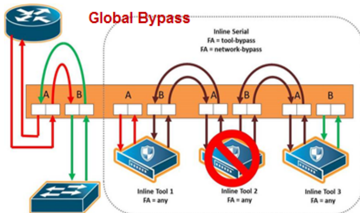
Figure 20-27: Inline Tool Series Global Bypass Failover Action
