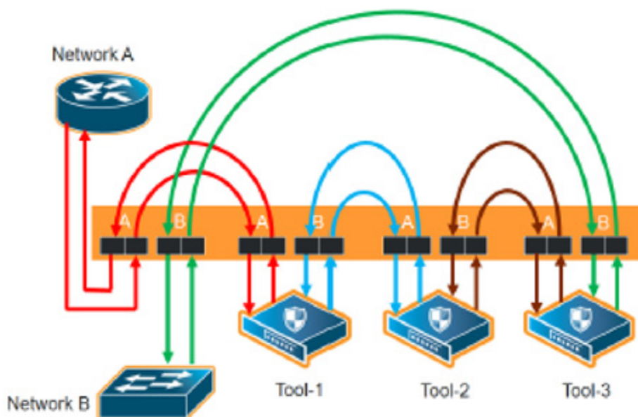
Figure 20-37: Inline Tool Series Per-Direction: Reversed
