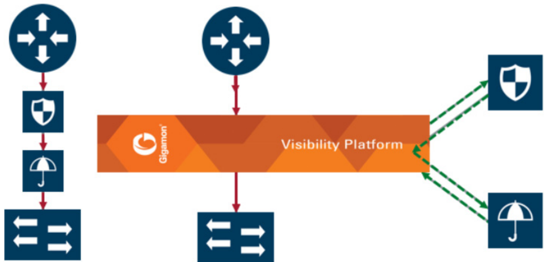
Figure 21-13: Serial Inline Tool Arrangement
