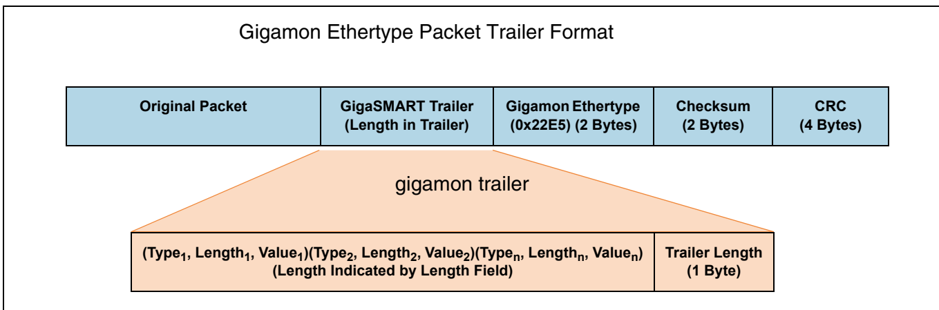
Figure 26-140: GigaSMART Trailer Format
