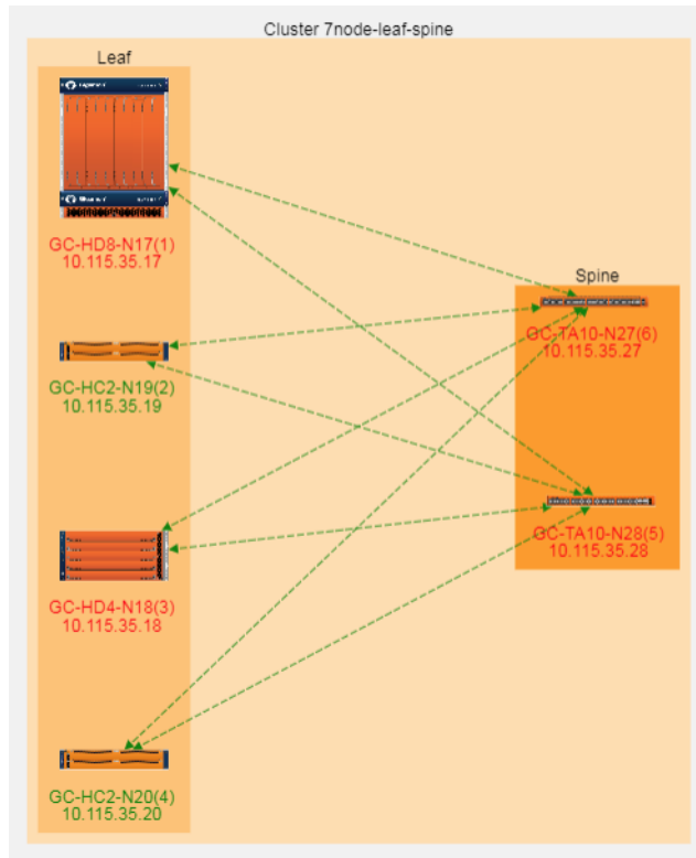
Figure 14-3: Leaf and Spine Topology
