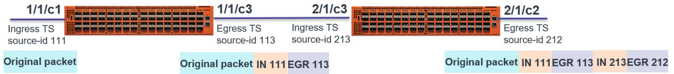
Figure 24-1: Timestamping
