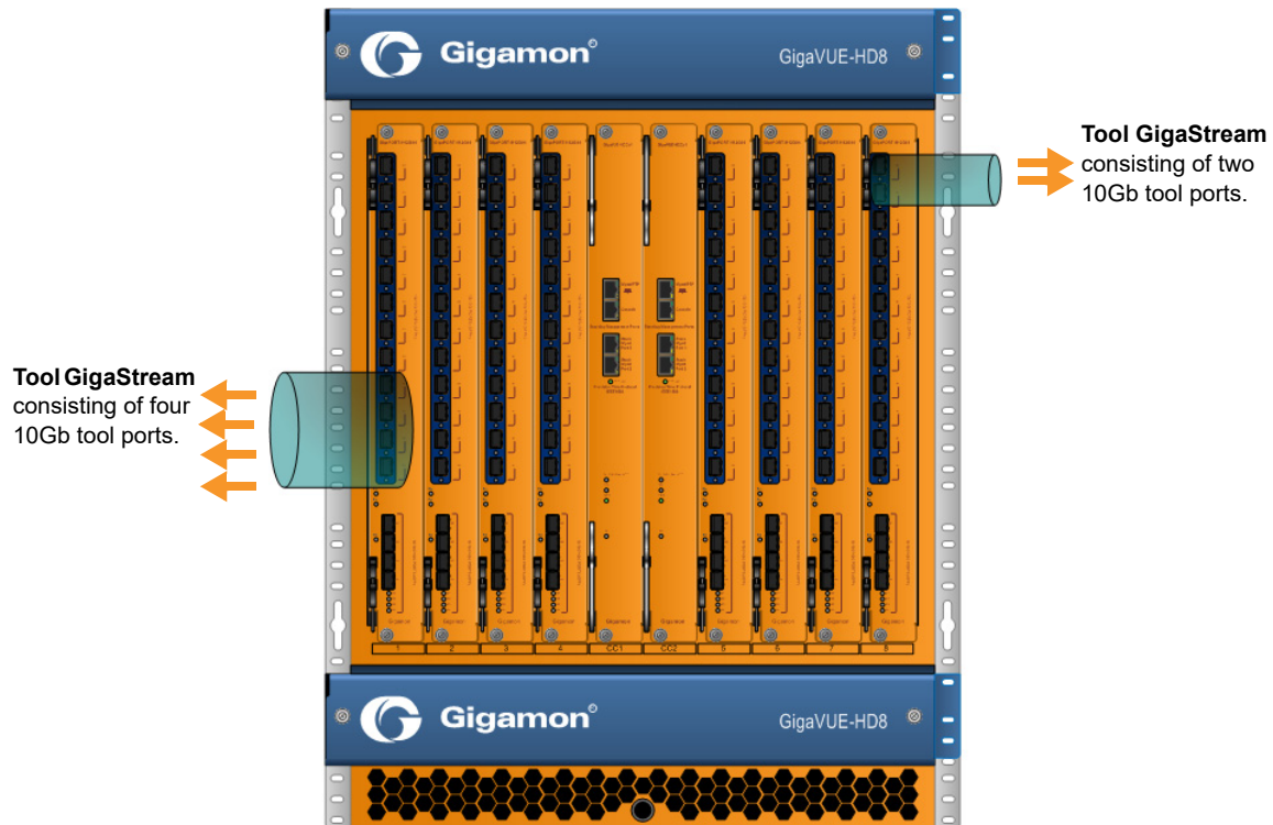
Figure 17-24: Regular Tool GigaStream Illustrated
