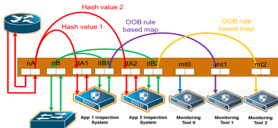
Figure 20-40: Out-of-Band Rule-Based Maps
