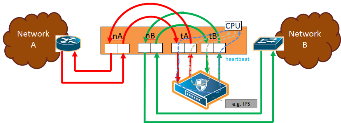
Figure 20-14: Traffic Path of To-Inline-Tool
